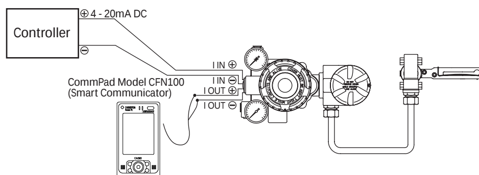
Figure 1 Wiring for model AVP200
