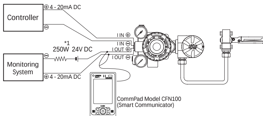
Figure 2 Wiring for model AVP201
